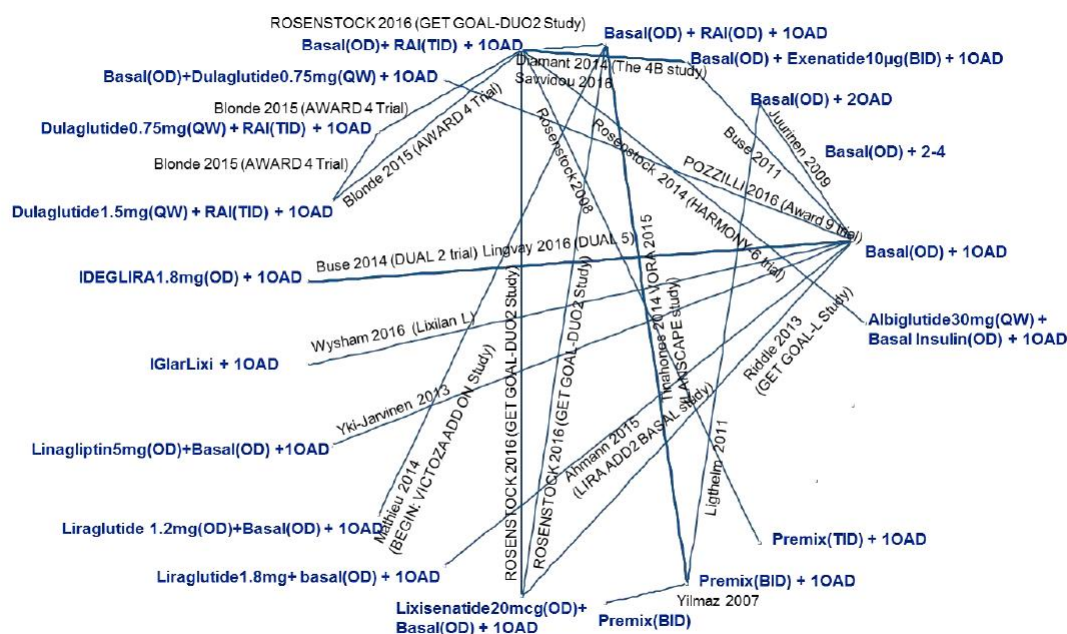
Figure 10: Network Diagram for Change in Body Weight From Baseline Under the Bayesian Network Meta-Analysis Method
