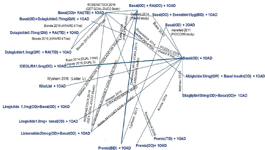
Figure 8: Network Diagram for Proportion of Patients With Less Than 7% A1C Under the Bayesian Network Meta-Analysis Method
